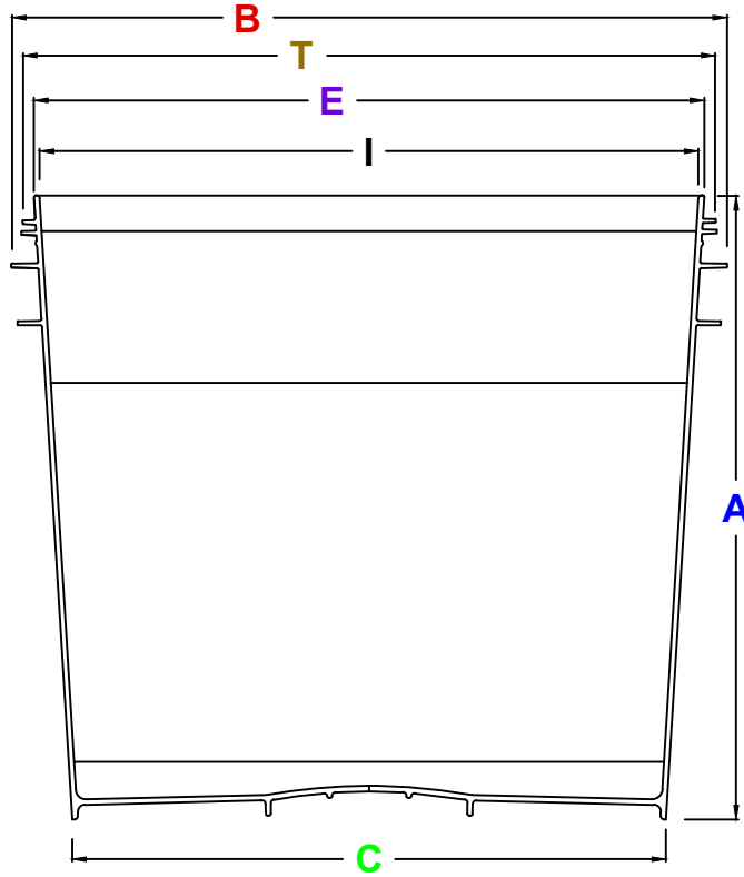
PAIL SECTION CUT VIEW
