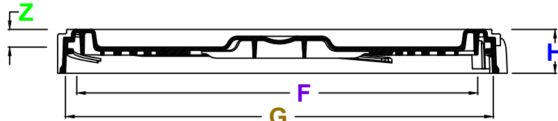
LID SECTION CUT VIEW
